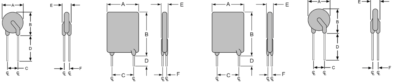
Figure 1 Lead Size: 24AWG Φ 0.51 mm Diameter
