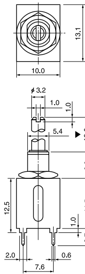
KS□□□□S SHAFT TYPE SUPPORT 부착 (V형 P/C MOUNT용)
